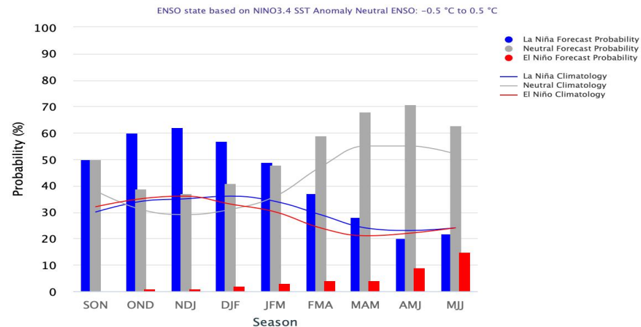
Mid-September 2024 IRI Model-Based Probabilistic ENSO Forecasts
