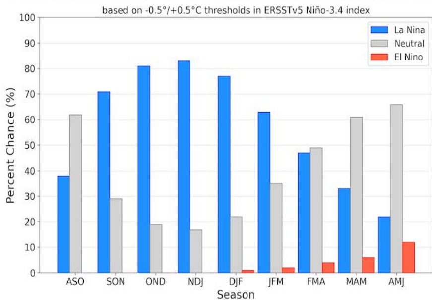
Official NOAA CPC ENSO Probabilities (issued September 2024)
